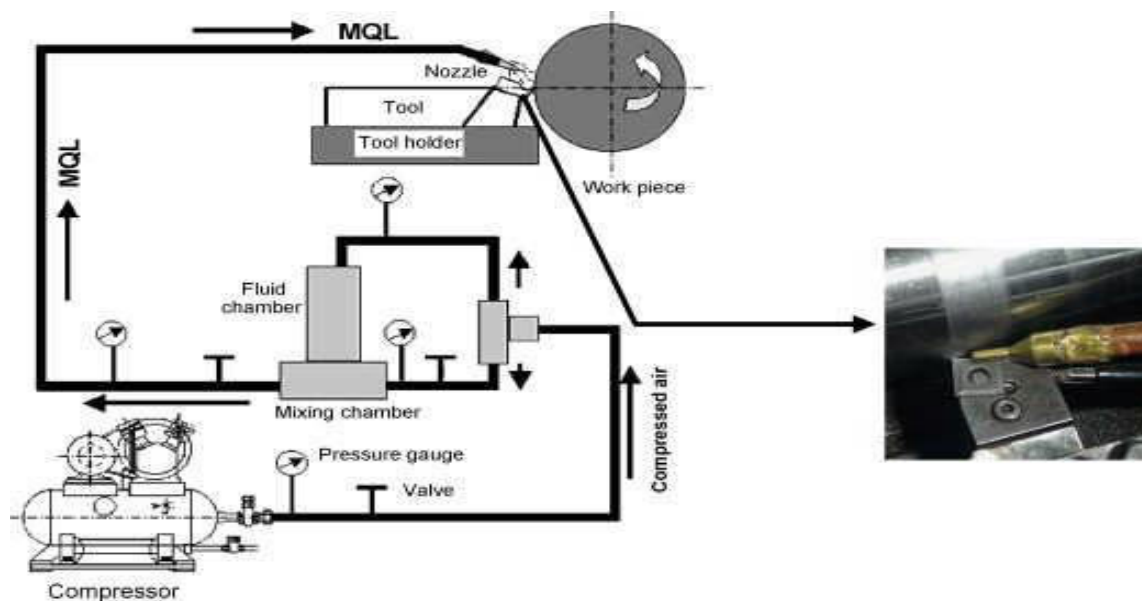
Figure 1: Typical schematic view of MQL unit
