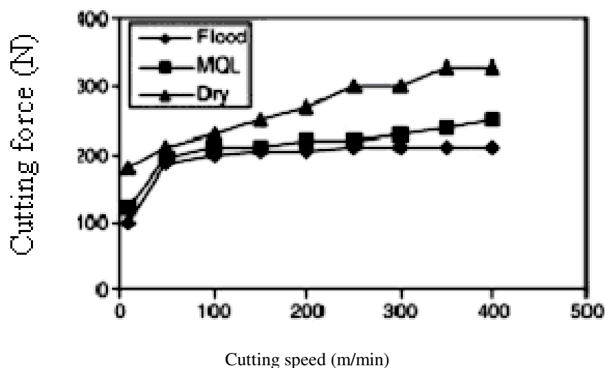
Figure 8: Variation cutting force with cutting speed.
